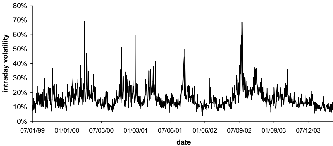
Figure 4: Estimated (realized) volatilities over the sample period July, 1999, until December, 2003, for the S&P500 index.
