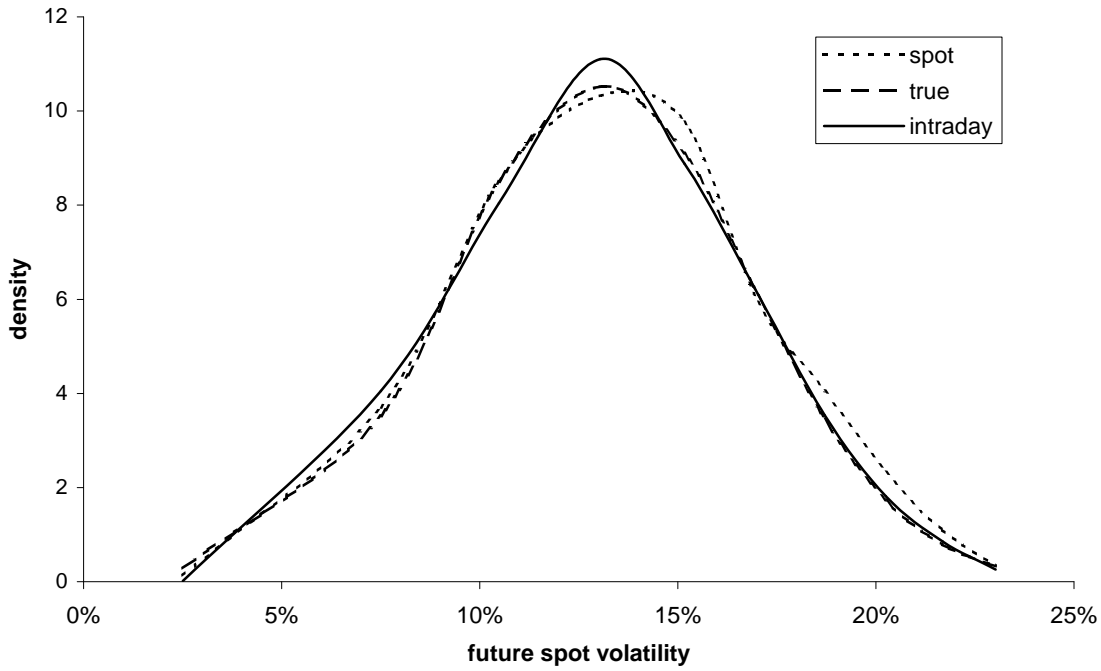
Figure 3: Estimated risk-neutral volatility distribution over a horizon of one month based on five years of simulated data in the Heston (1993) model with the Pan (2002) parameters. The solid line denotes the estimate based on realized intraday volatilities. The dotted line shows the estimate based on the actual spot volatilities. The dashed line shows the theoretical risk-neutral volatility distribution. All distributions are conditional on an average initial level of spot volatility \sigma_t = 12.4\% .
